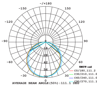
LNI617TV-W8-24V-RGBW30K-5.2-FT-F-OW-F-OW LINIO NEON 1617 TV RGBW, Vertical bend, RGBW30K, 5.18W/ft
