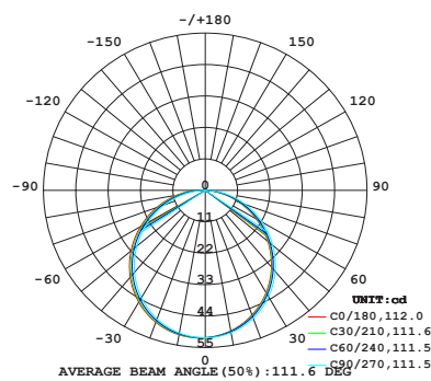
LNI617SV-W8-24V-RGBW30K-5.2-FT-F-OW-F-OW LINIO NEON 1617 SV RGBW, Horizontal bend, RGBW30K, 5.18W/ft
