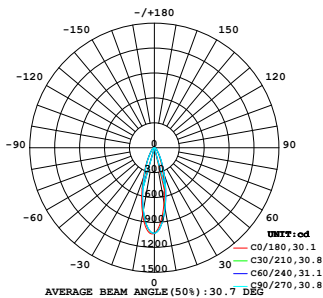
Zonal Lumen Summary
