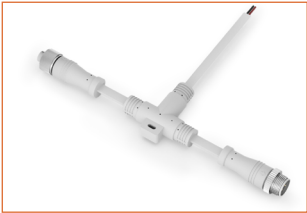
MFTCW-5P-67 Male and female T-shaped connector, white cable, 5 pin, IP67, Wet
