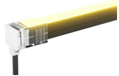
LNI615-MEC3-B-2P Mechanical end cap without screws, bottom entry with 0.98' (30cm) cable, 2 pin
